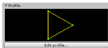
Fig. 5 Profile preview
