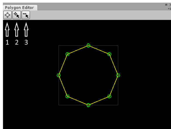
Fig. 6 Polygon Editor
